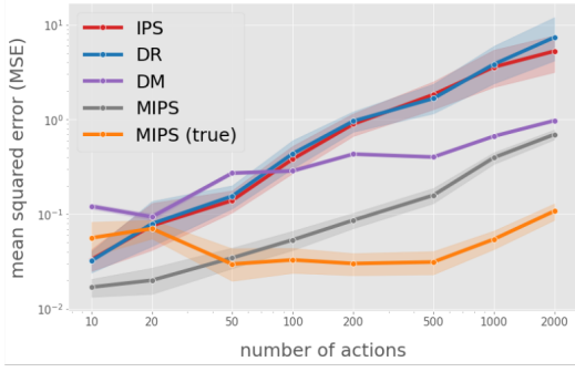
Figure 2. MSE (on log-scale) with varying number of actions.
