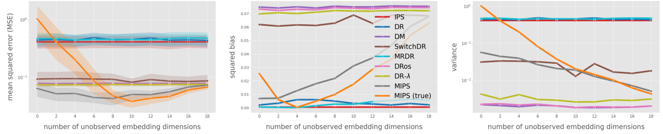
Figure 12. MSE, Squared Bias, and Variance with varying number of unobserved dimensions in action embeddings
