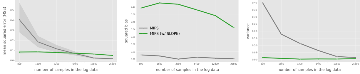
Figure 5. MSE, Squared Bias, and Variance of MIPS with or without data-driven action embedding selection (SLOPE).
