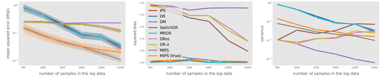
Figure 27. MSE, Squared Bias, and Variance with varying sample size
