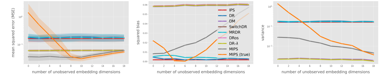
Figure 28. MSE, Squared Bias, and Variance with varying number of unobserved dimensions in action embeddings
