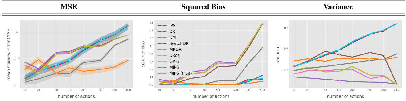
Figure 26. MSE, Squared Bias, and Variance with varying number of actions
