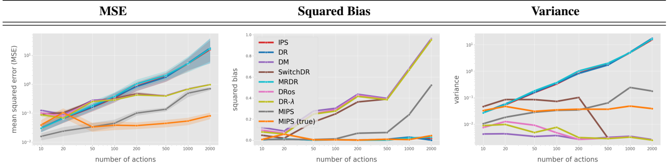
Figure 10. MSE, Squared Bias, and Variance with varying number of actions
