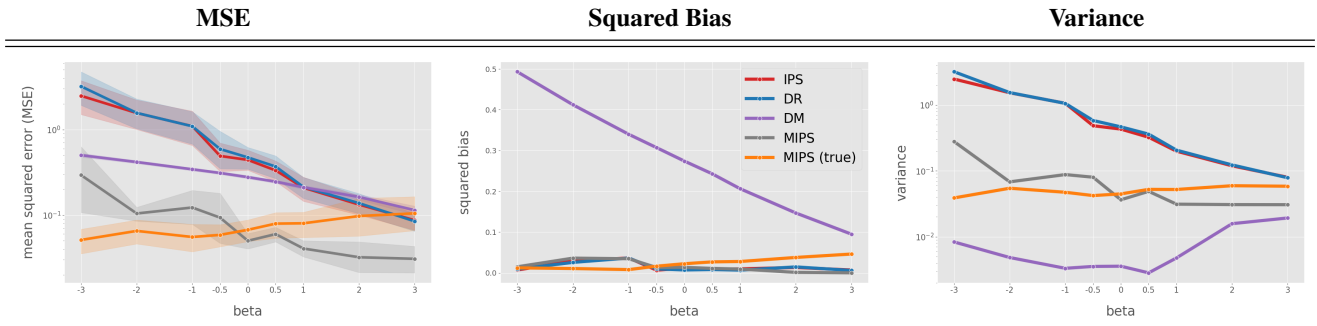
Figure 7. MSE, Squared Bias, and Variance with varying logging policies ( \beta_0 )
