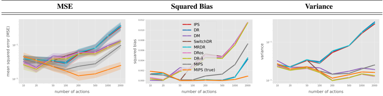
Figure 22. MSE, Squared Bias, and Variance with varying number of actions
