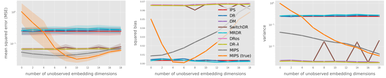
Figure 20. MSE, Squared Bias, and Variance with varying number of unobserved dimensions in action embeddings
