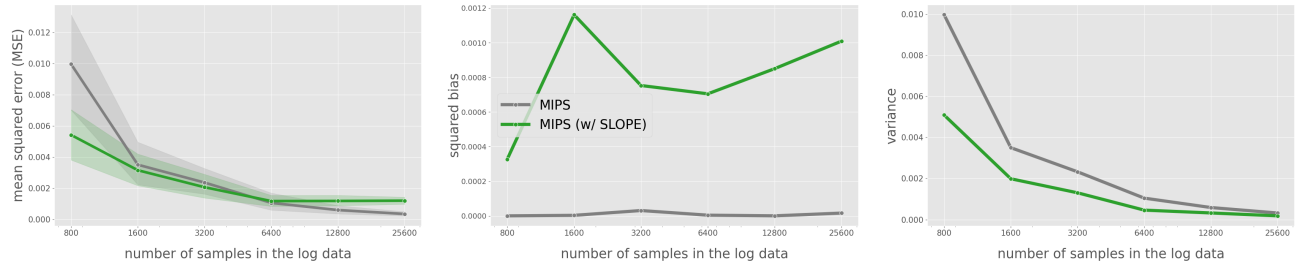
Figure 25. MSE, Squared Bias, and Variance of MIPS with or without data-driven action embedding selection (using SLOPE)
