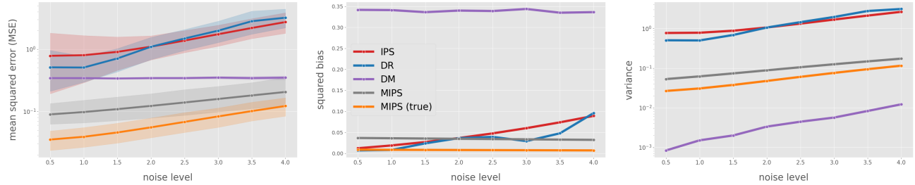
Figure 9. MSE, Squared Bias, and Variance with varying noise levels ( \sigma )
