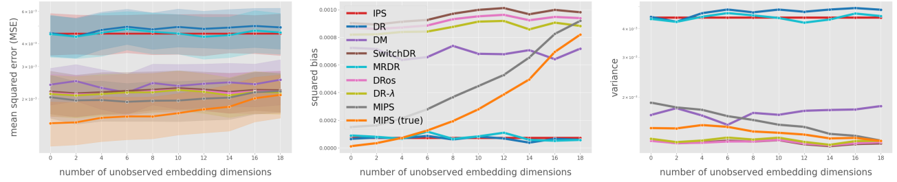
Figure 24. MSE, Squared Bias, and Variance with varying number of unobserved dimensions in action embeddings
