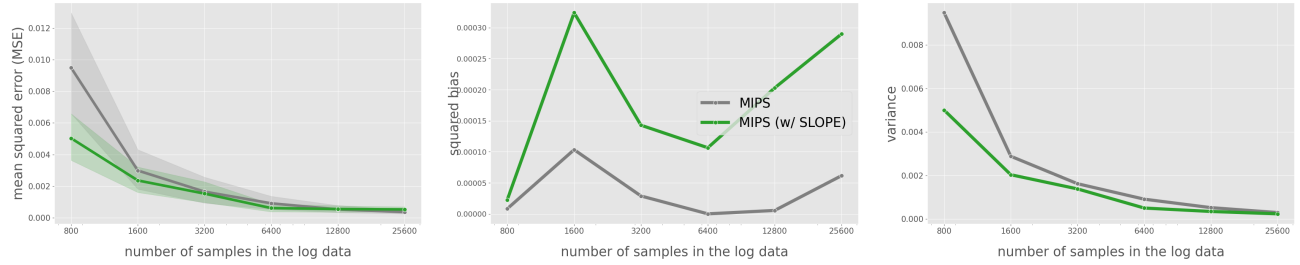
Figure 33. MSE, Squared Bias, and Variance of MIPS with or without data-driven action embedding selection (using SLOPE)
