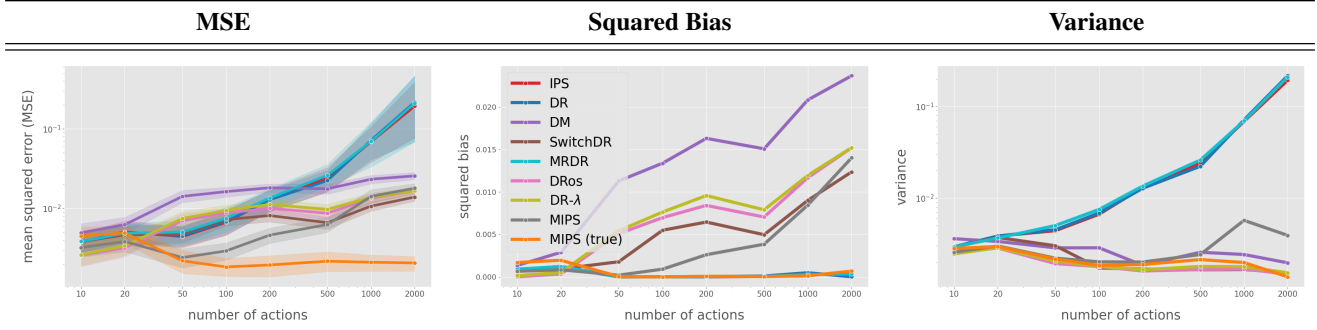
Figure 14. MSE, Squared Bias, and Variance with varying number of actions
