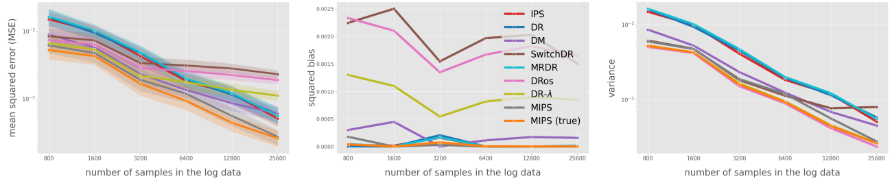
Figure 31. MSE, Squared Bias, and Variance with varying sample size
