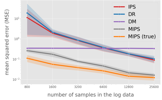
Figure 3. MSE (on log-scale) with varying number of samples.
