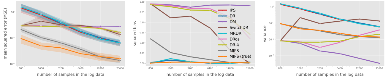
Figure 19. MSE, Squared Bias, and Variance with varying sample size
