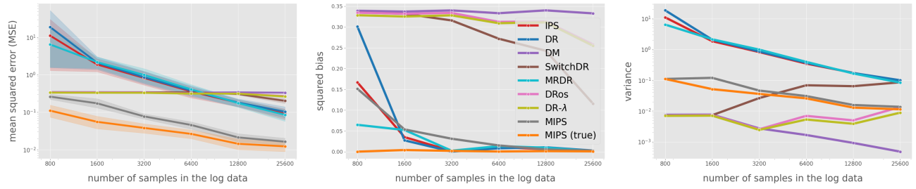
Figure 11. MSE, Squared Bias, and Variance with varying sample size
