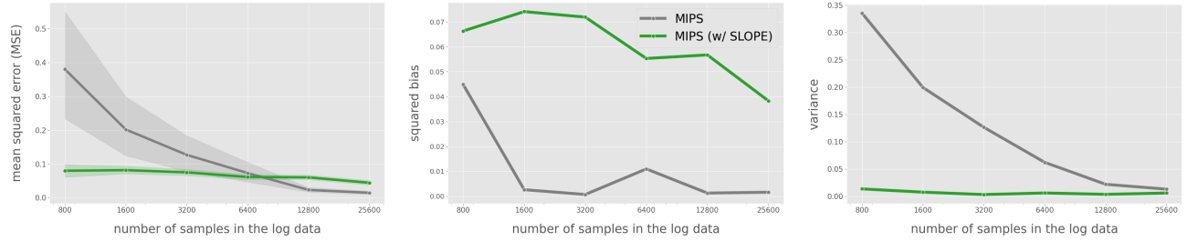
Figure 13. MSE, Squared Bias, and Variance of MIPS with or without data-driven action embedding selection (using SLOPE)
