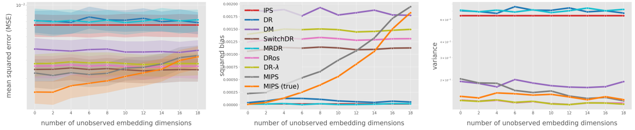
Figure 16. MSE, Squared Bias, and Variance with varying number of unobserved dimensions in action embeddings
