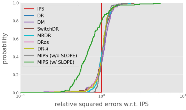
Figure 6. CDF of relative squared error w.r.t. IPS.
