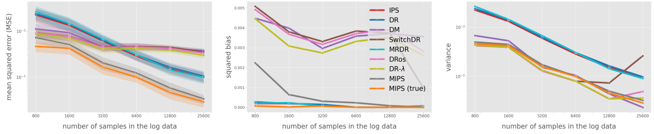
Figure 23. MSE, Squared Bias, and Variance with varying sample size
