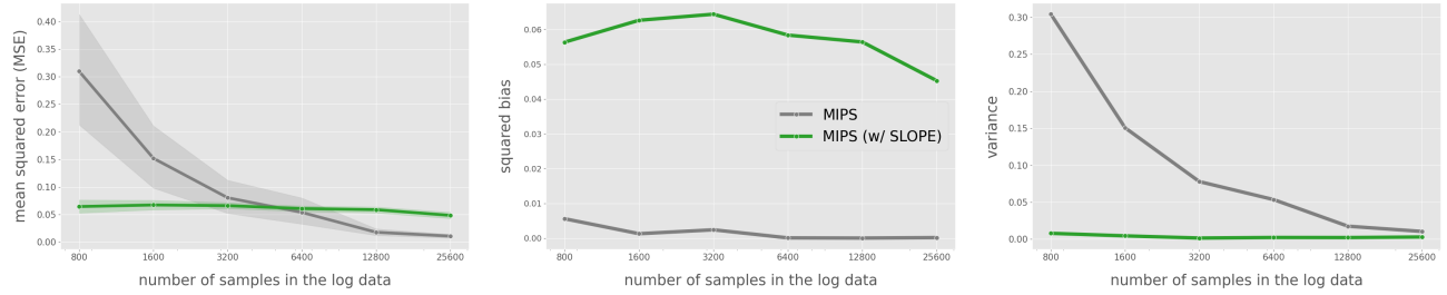
Figure 21. MSE, Squared Bias, and Variance of MIPS with or without data-driven action embedding selection (using SLOPE)
