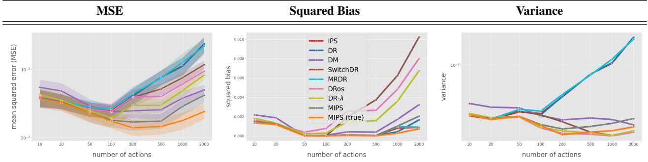
Figure 30. MSE, Squared Bias, and Variance with varying number of actions
