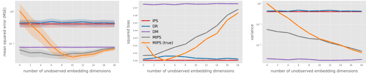
Figure 4. MSE, Squared Bias, and Variance with varying number of unobserved dimensions in action embeddings.
