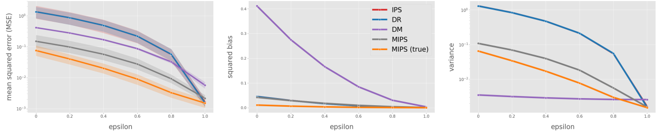
Figure 8. MSE, Squared Bias, and Variance with varying evaluation policies ( \epsilon )
