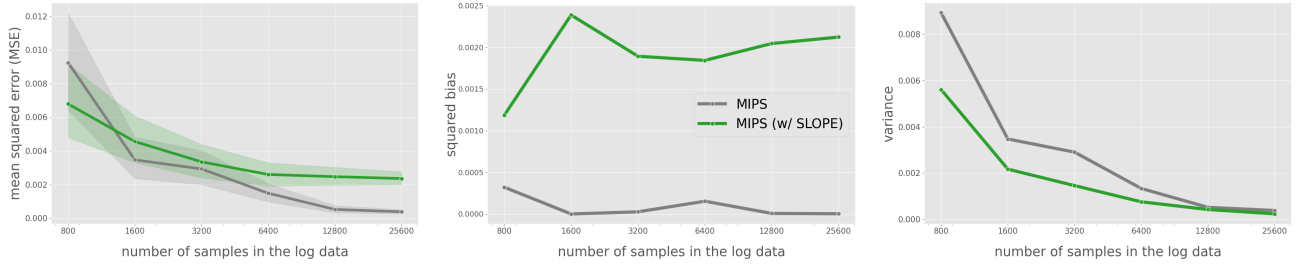
Figure 17. MSE, Squared Bias, and Variance of MIPS with or without data-driven action embedding selection (using SLOPE)
