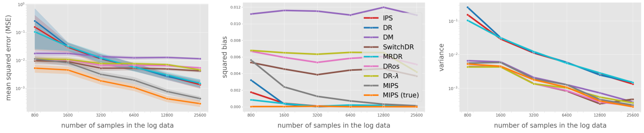
Figure 15. MSE, Squared Bias, and Variance with varying sample size
