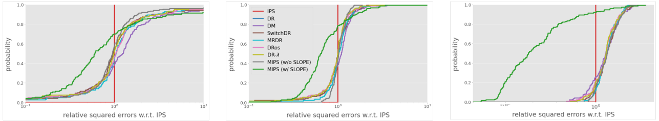
Figure 34. CDF of squared errors relative to IPS with different sample sizes (From left to right, n = 10000, 50000, 500000 ). CDFs are estimated with 150 different sets of bootstrapped logged bandit data. Note that the x-axis is reported on log-scale.
