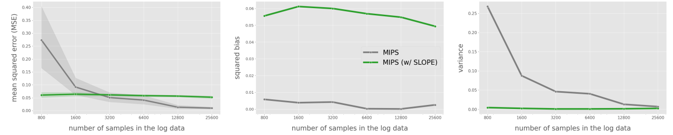
Figure 29. MSE, Squared Bias, and Variance of MIPS with or without data-driven action embedding selection (using SLOPE)
