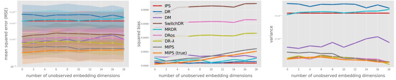
Figure 32. MSE, Squared Bias, and Variance with varying number of unobserved dimensions in action embeddings
