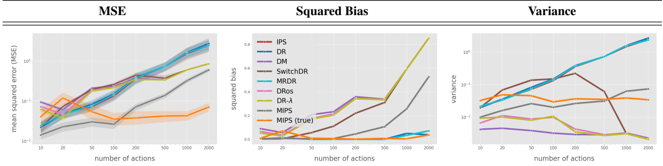
Figure 18. MSE, Squared Bias, and Variance with varying number of actions
